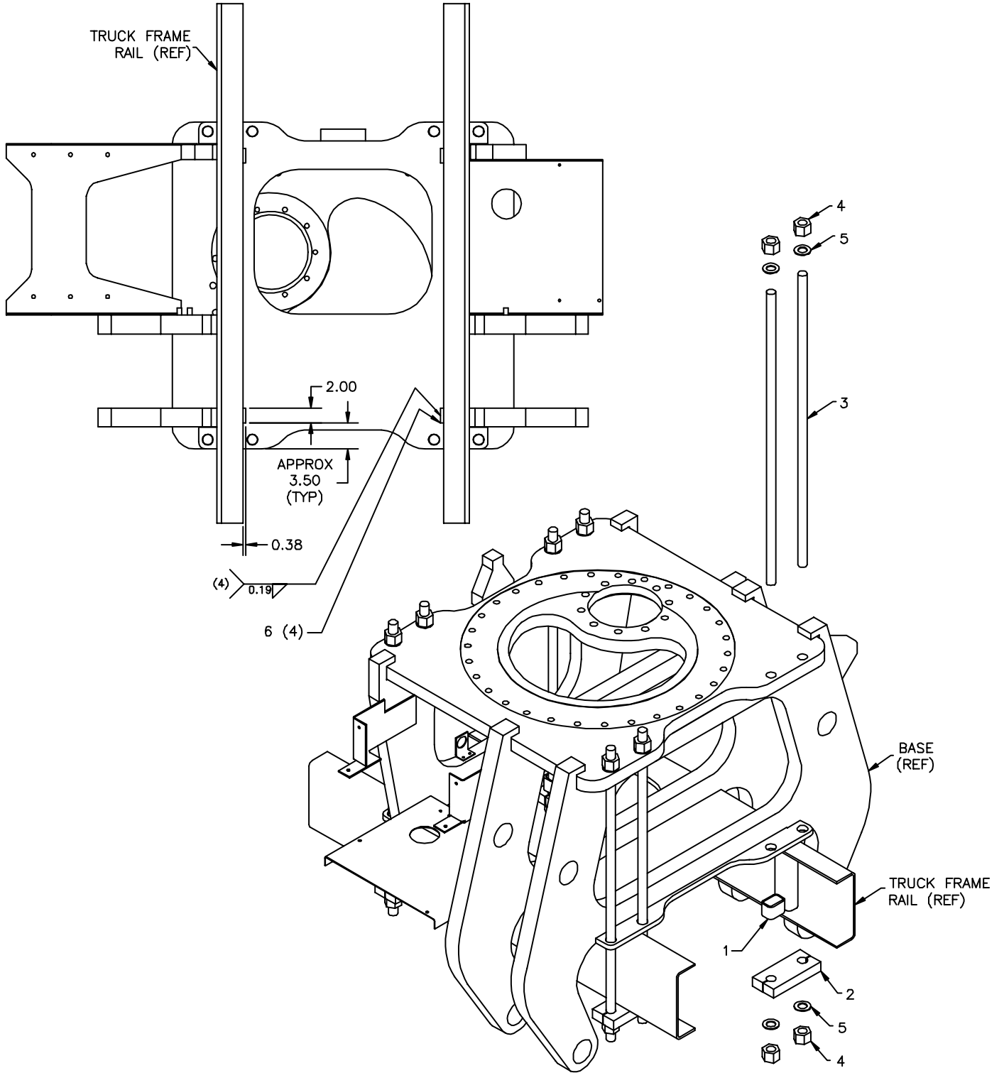
BOTTOM VIEW
